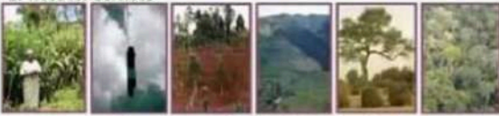
soil fertility carbon sequestration soil erosion watershed protection shade biodiversity
